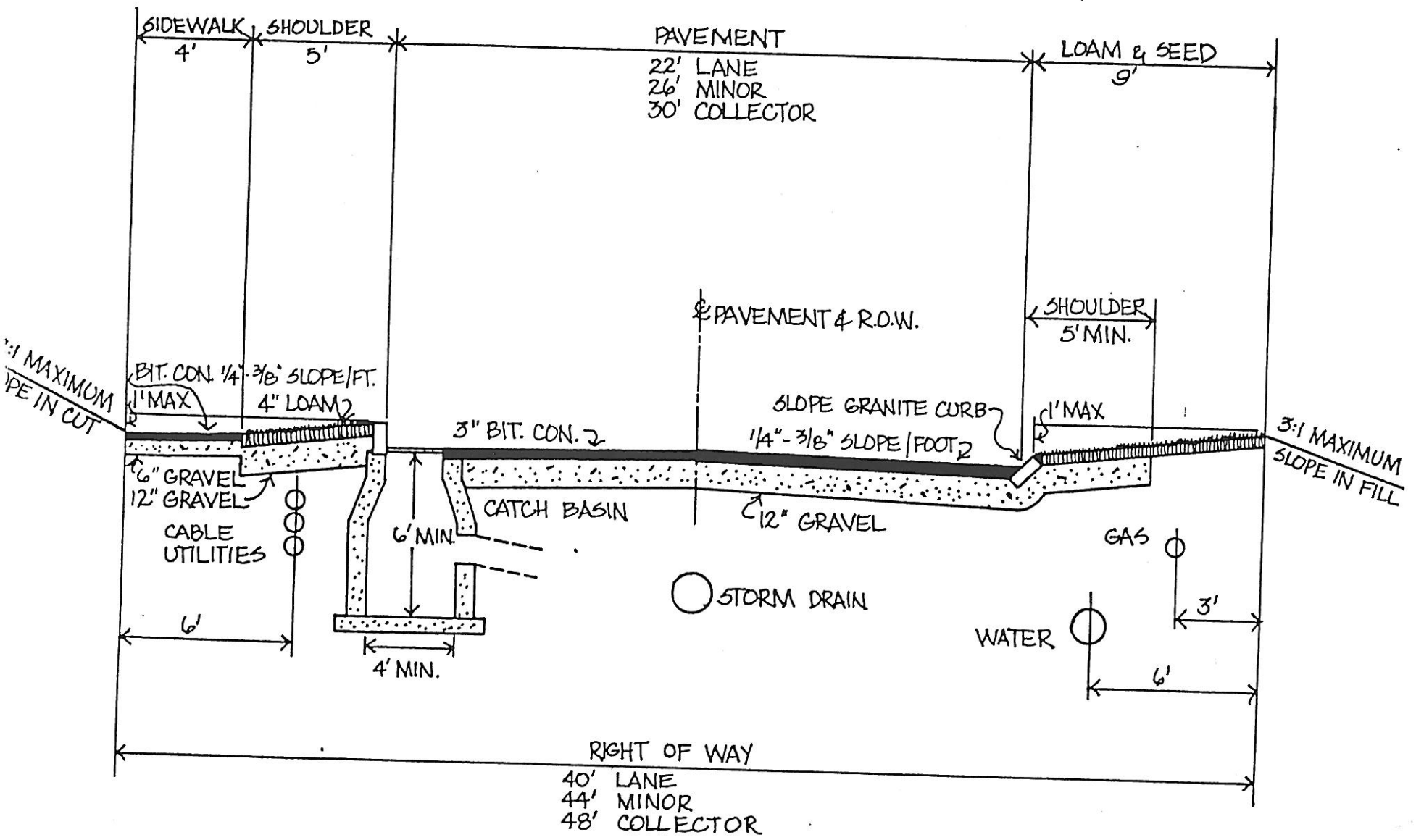
FIGURE 1 . TYPICAL STREET CROSS SECTION LITTLETON PLANNING BOARD HERR ASSOCIATES May 10, 1978 NOT TO SCALE
