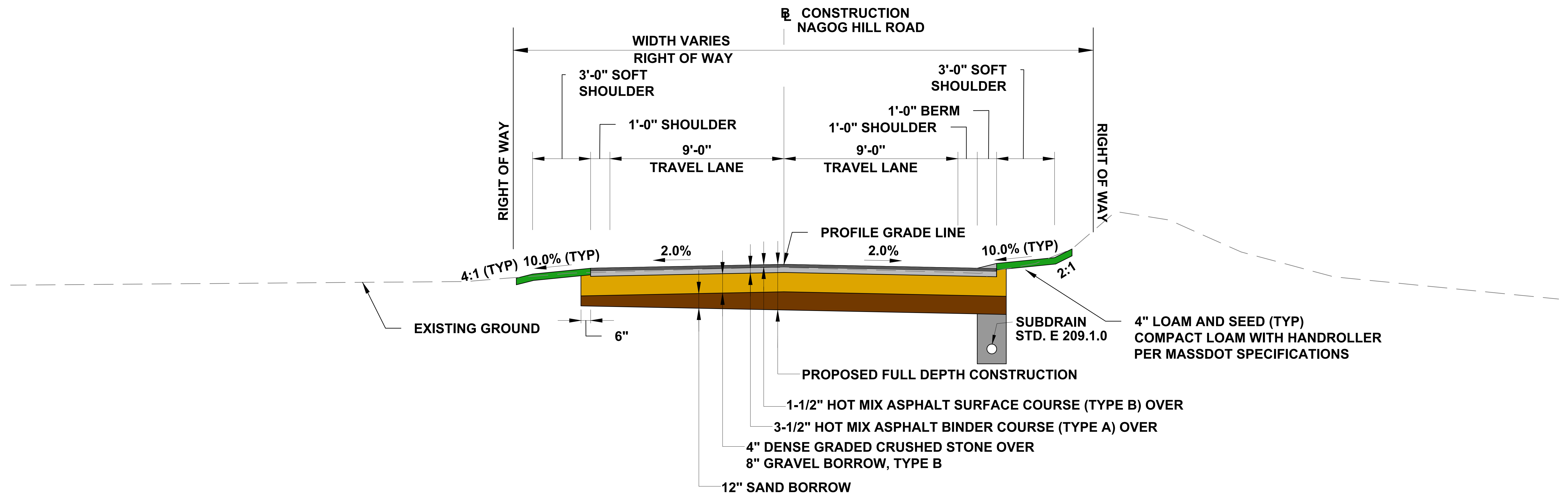
TYPICAL SECTION NAGOG HILL ROAD
