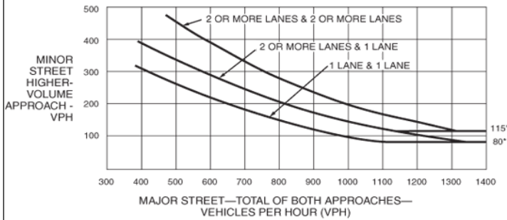
Figure 4C-1. Warrant 2, Four-Hour Vehicular Volume
