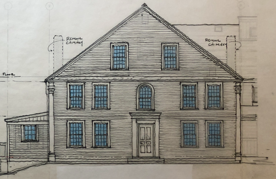
EXISTING STRUCTURE — 4 UNITS HOUSING — STREET ELEVATION
