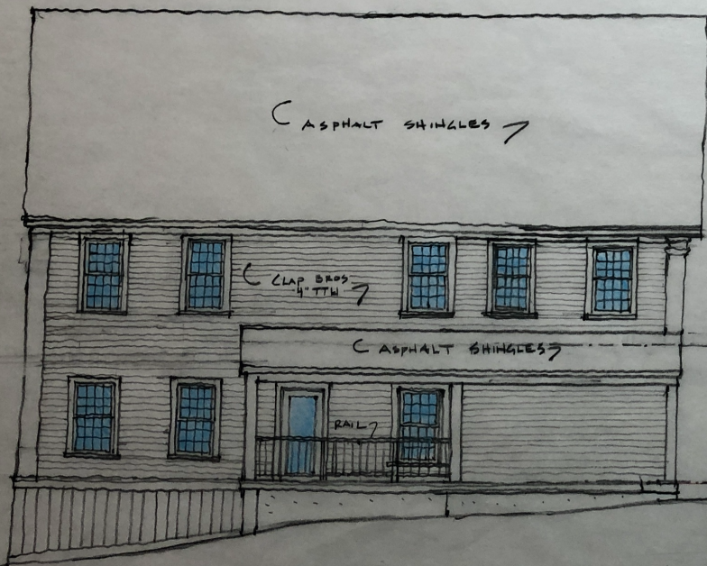
NEW STRUCTURE — 4 UNITS HOUSING — SIDE ELEVATION
