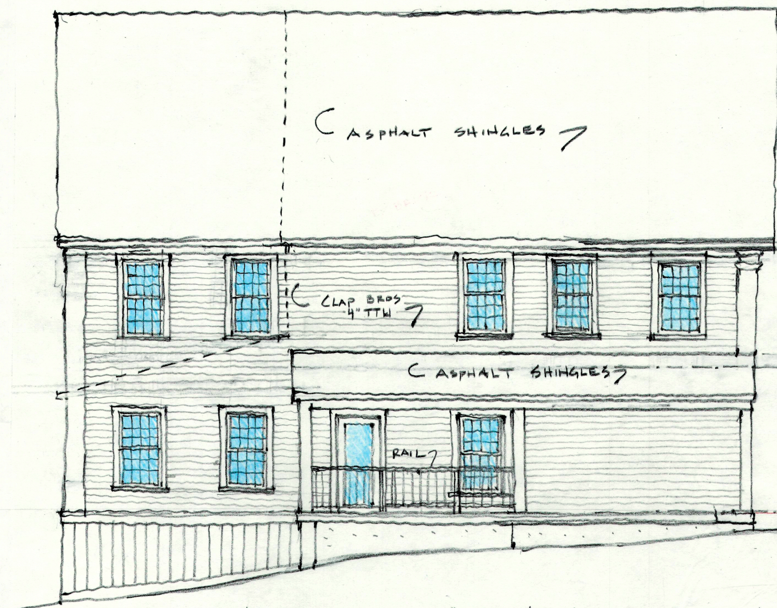
NEW STRUCTURE — 4 UNITS HOUSING — SIDE ELEVATION
