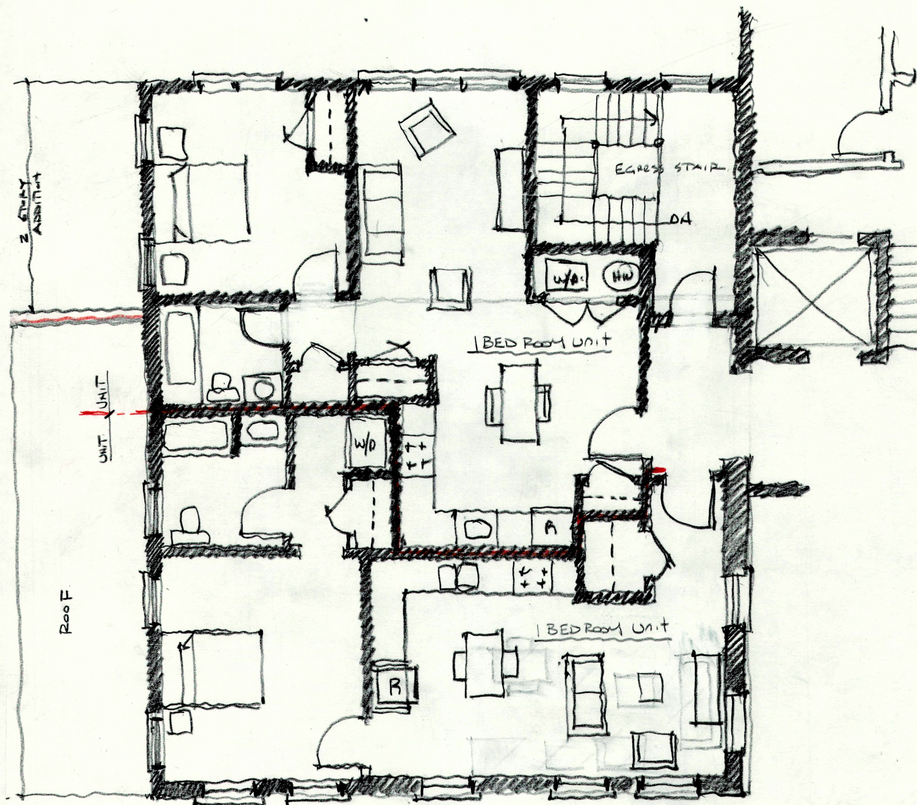
Second Floor Plan Existing or New Building
