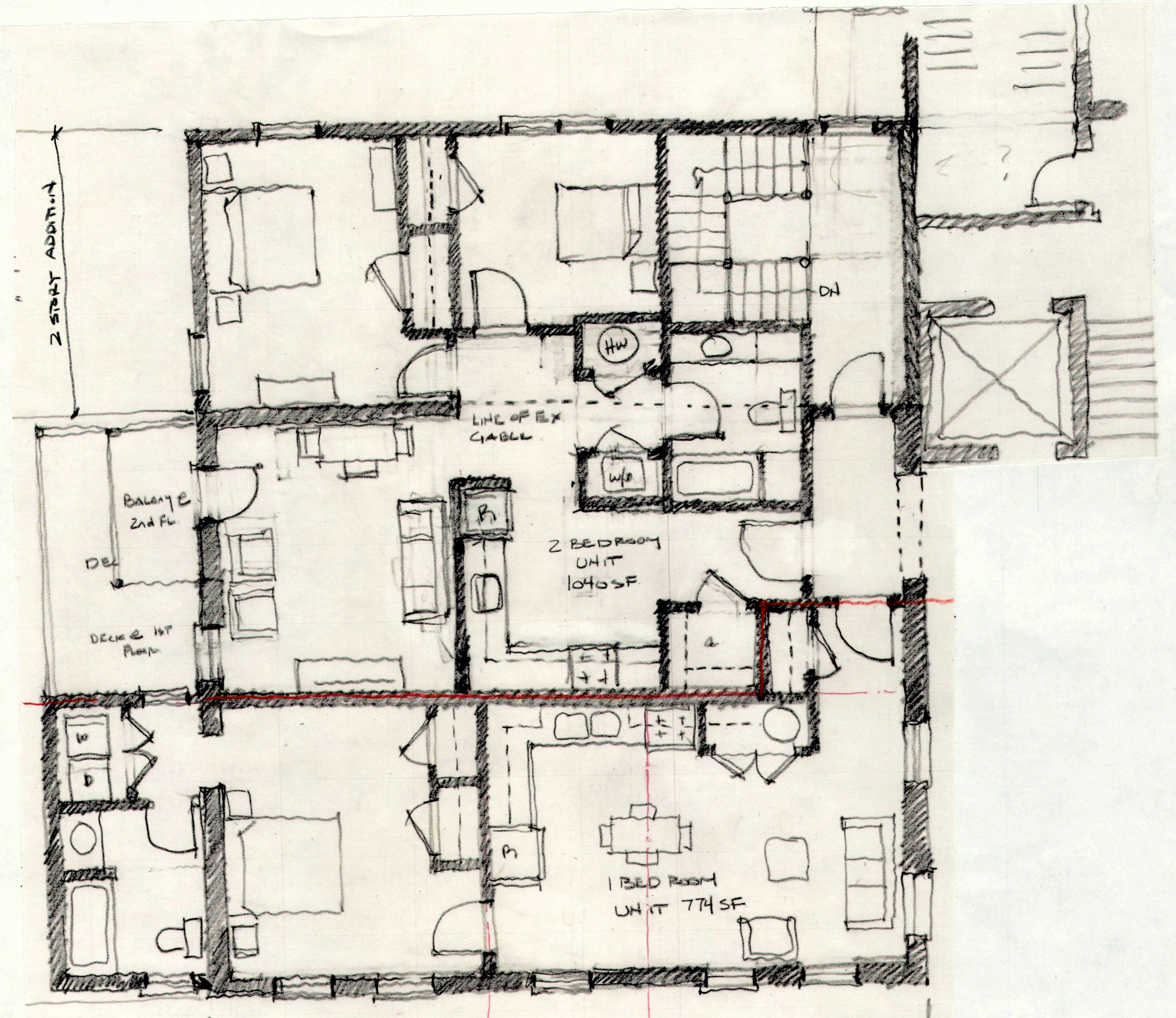
First Floor Plan Existing or New Building
