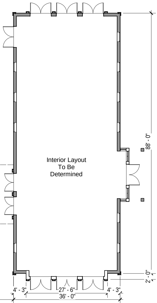
First Floor Plan Building D - 3,204 SF
