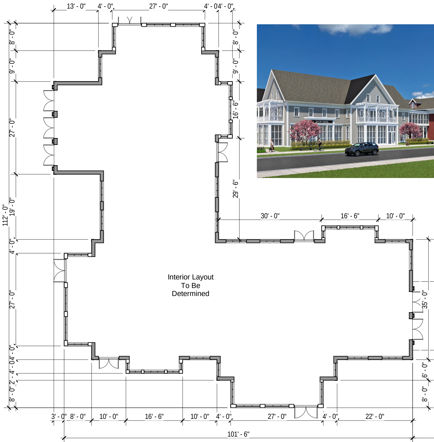
First Floor Plan Building C - 6,595 SF
