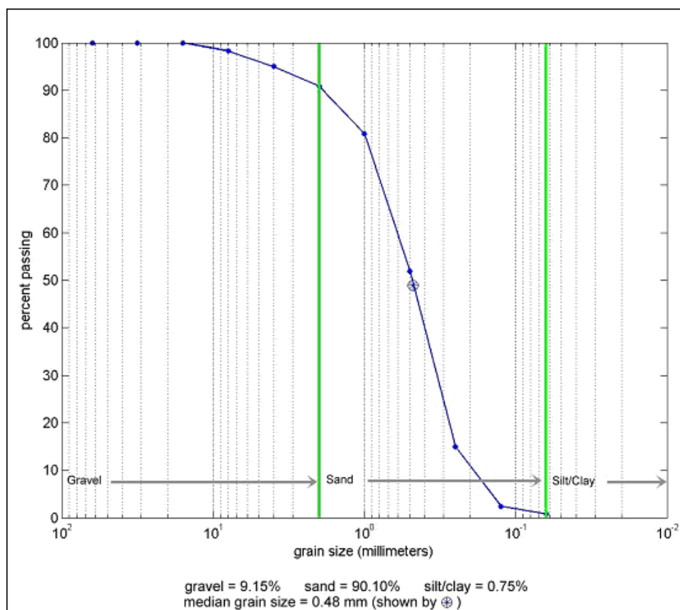
Figure B3. Example of a grain size analysis curve.
